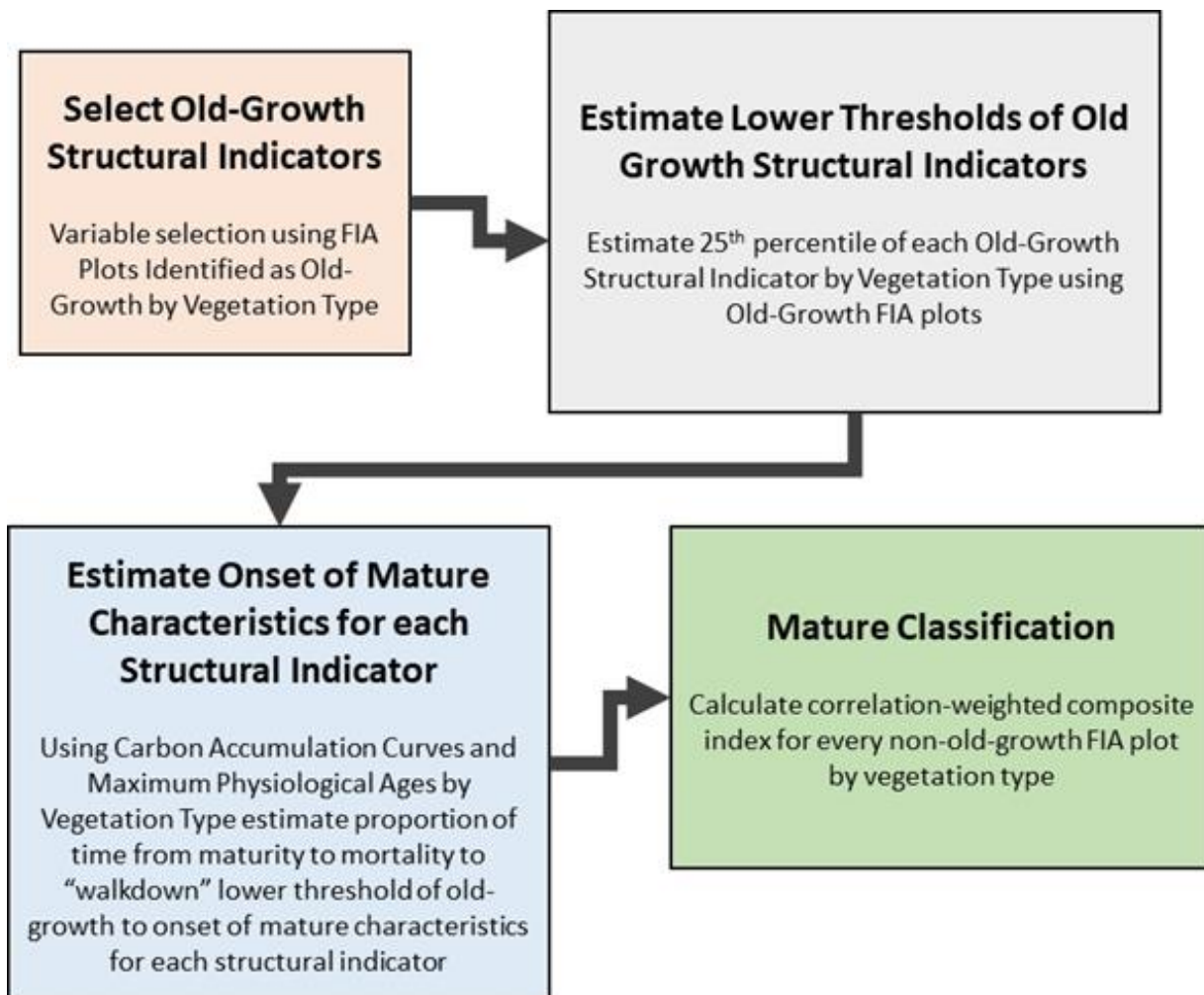
Figure 2.—Fundamental components of the FIGSS approach (Woodall et al. in preparation) include selecting old-growth structural indicators that are used to identify the lower thresholds of old-growth attributes, then using a walkdown factor to identify the onset of mature forest conditions. The definitions are then applied non-old-growth plots to classify mature forest.
