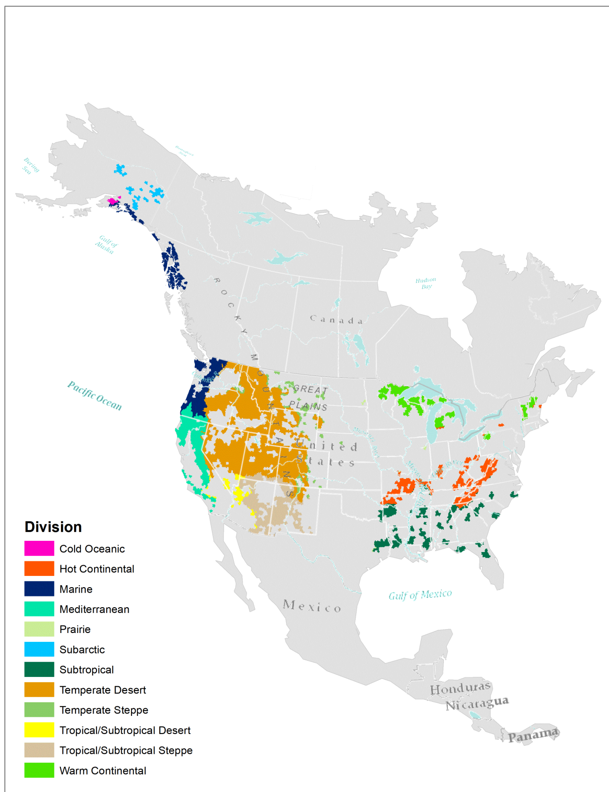
Figure A3.3.—Fireshed map of ecological divisions.
